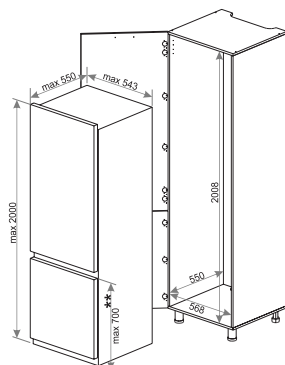
П600х (2140)**
