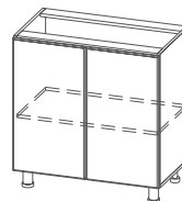
C550/C600/C700/C800* 550/600/700/800x824x506мм
