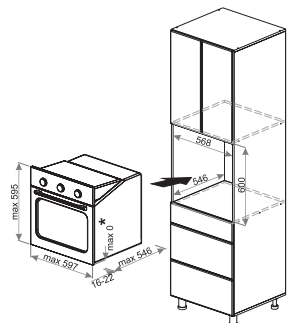
П600, П600я (2140/2332)*
