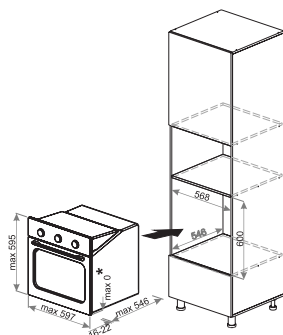
П600дм (2140/2332)*
